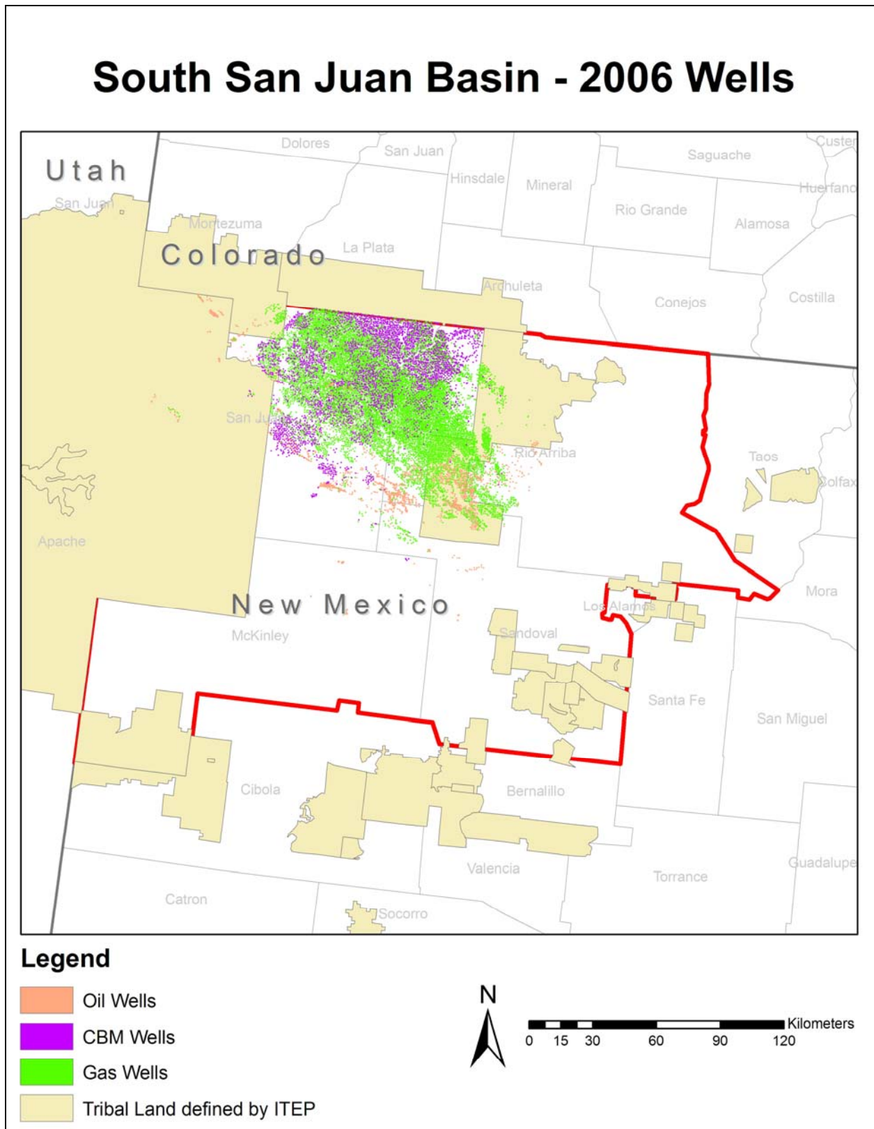
Figure 1. South San Juan Basin boundaries overlaid with 2006 oil and gas well locations. 1
