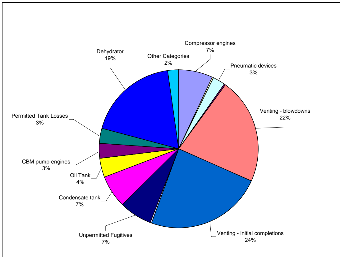
Figure 7. South San Juan Basin VOC emissions proportional contributions by source category.
