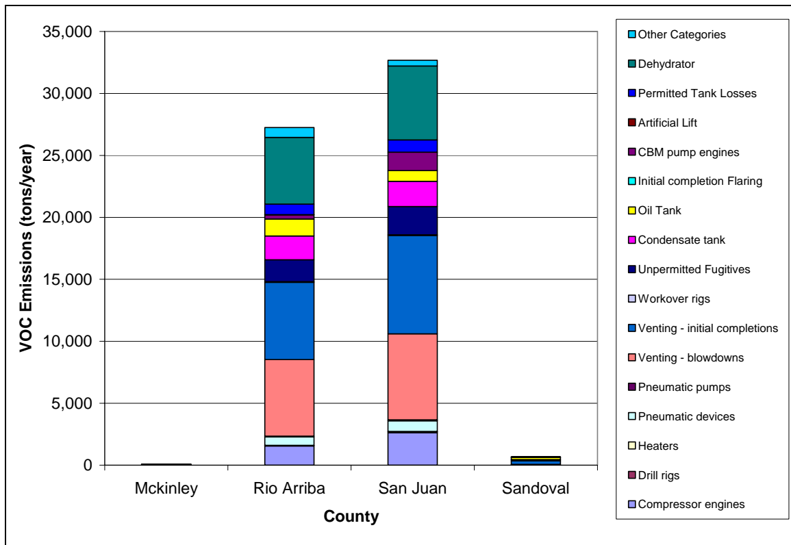
Figure 4. 2006 VOC emissions by source category and by county in the South San Juan Basin.
