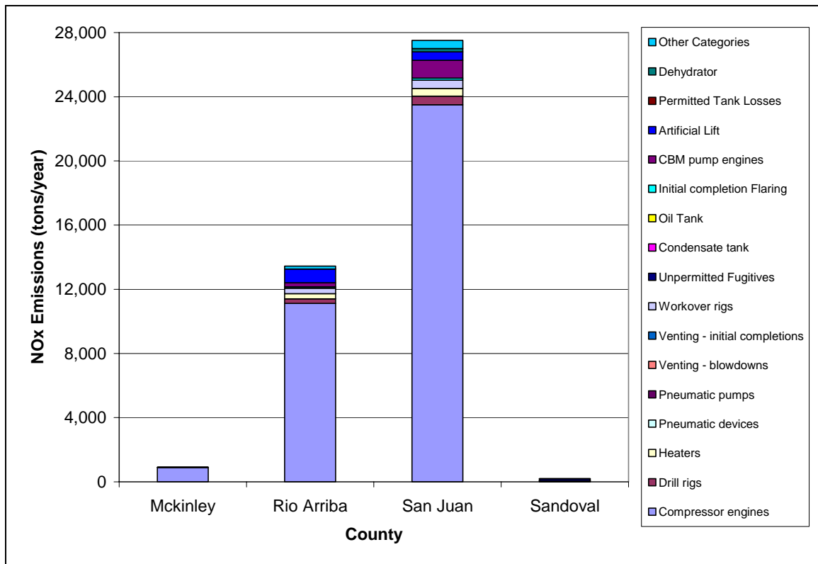
Figure 2. 2006 NOx emissions by source category and by county in the South San Juan Basin.
