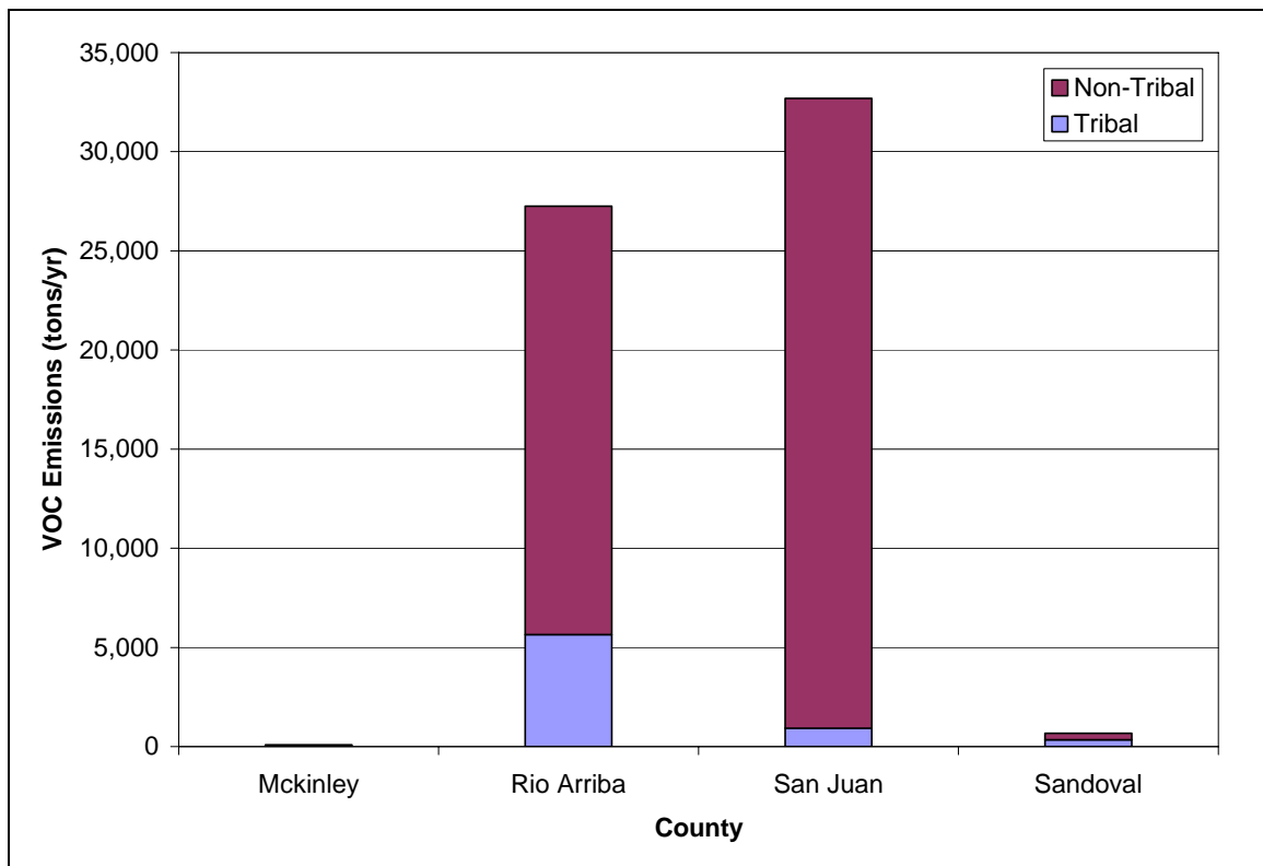
Figure 5. 2006 VOC emissions on tribal and non-tribal land by county in the South San Juan Basin.
