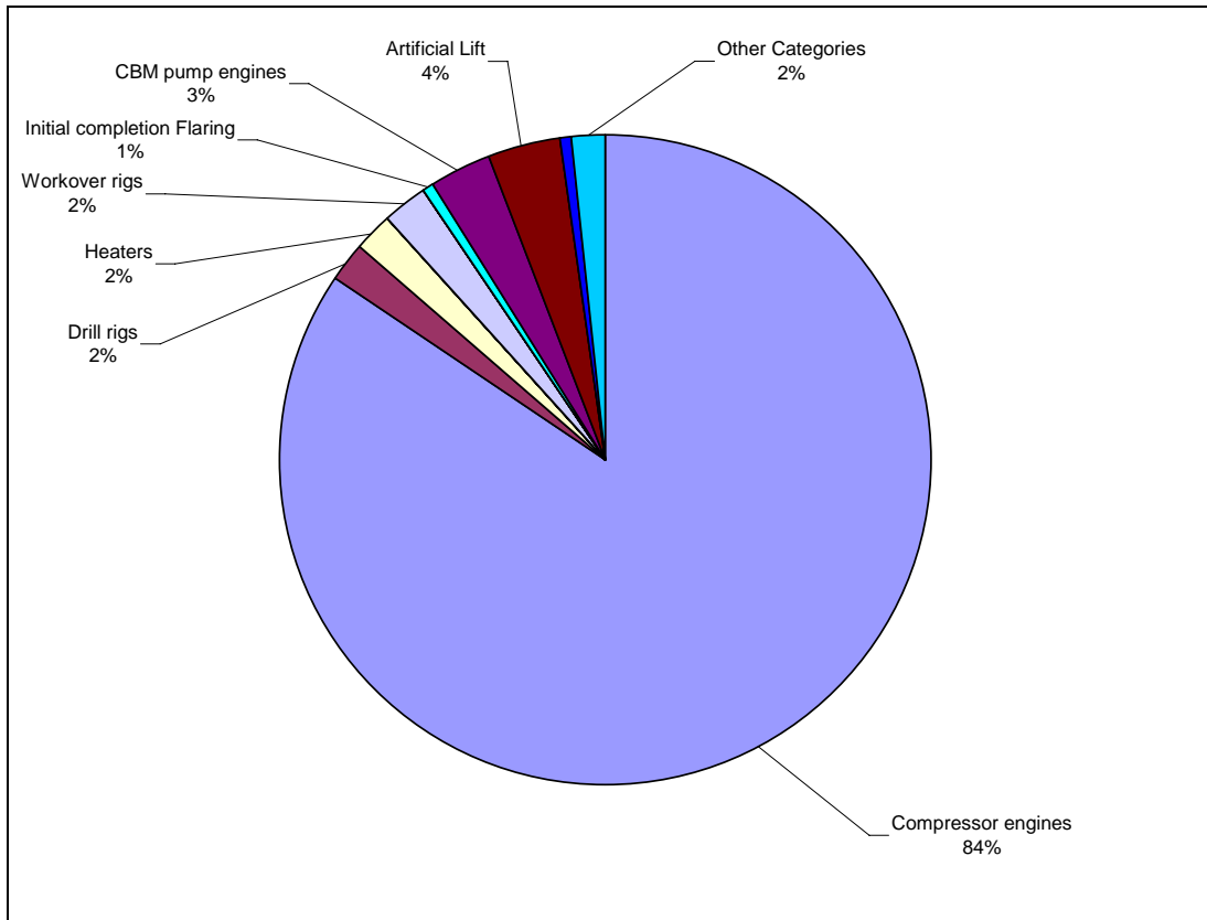
Figure 6. South San Juan Basin NOx emissions proportional contributions by source category.
