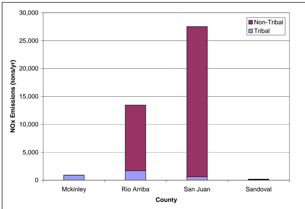
Figure 3. 2006 NOx emissions on tribal and non-tribal land by county in the South San Juan Basin.
