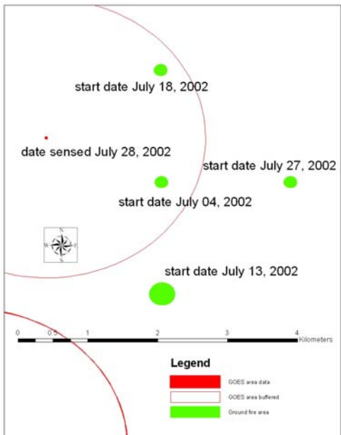
Figure 3. Enlarged view of ground data and GOES instantaneous fire size data demonstrating the proximity of the July 27 th and July 28 th detections (GOES spatial resolution 16 km 2 ). Even though GOES is most likely detecting this fire event, the data do not coincide.
