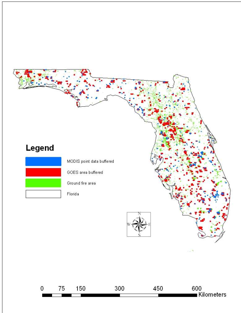
Figure 4. Coincidence in Florida ground fire area and the buffered GOES and MODIS products.
