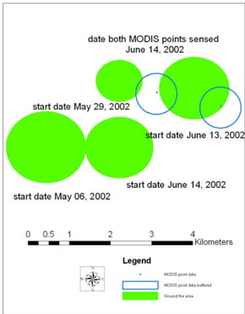
Figure 2. Enlarged view of ground data and MODIS point data demonstrating the proximity of the June 13 th and June 14 th detections (MODIS spatial resolution 1 km 2 ). Even though MODIS is most likely detecting these fire events, only 1 data point coincides.
