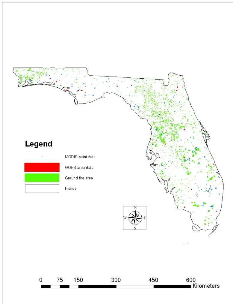
Figure 1. Coincidence in Florida ground fire area, GOES area and MODIS point data.
